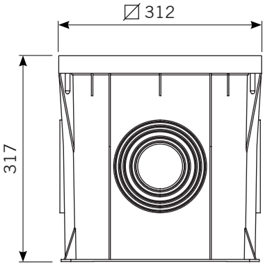
RECESS BOX
