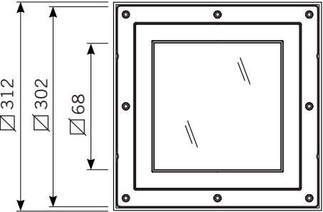
36 LED VERSION
